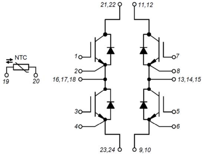
Figure 14. Circuit Diagram
