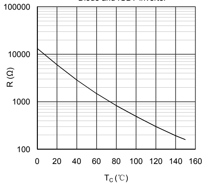
Figure 13. NTC Characteristics
