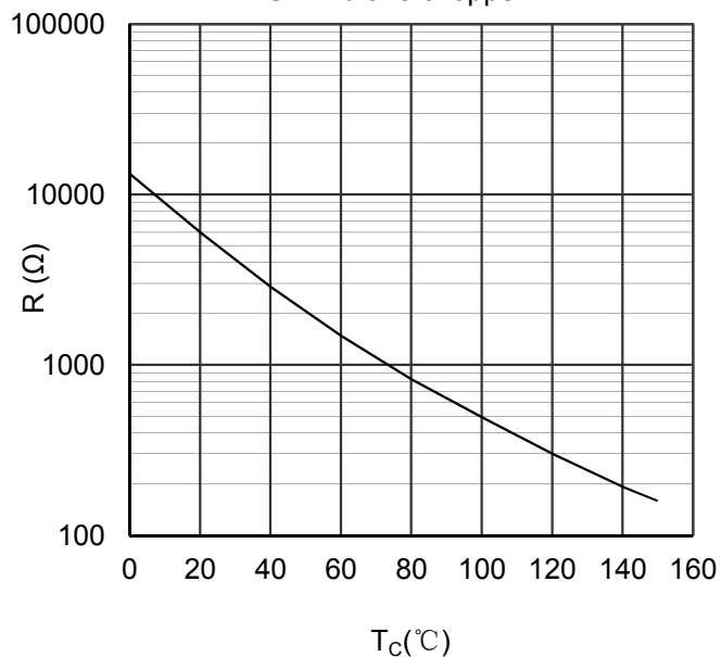
Figure 14. NTC Characteristics
