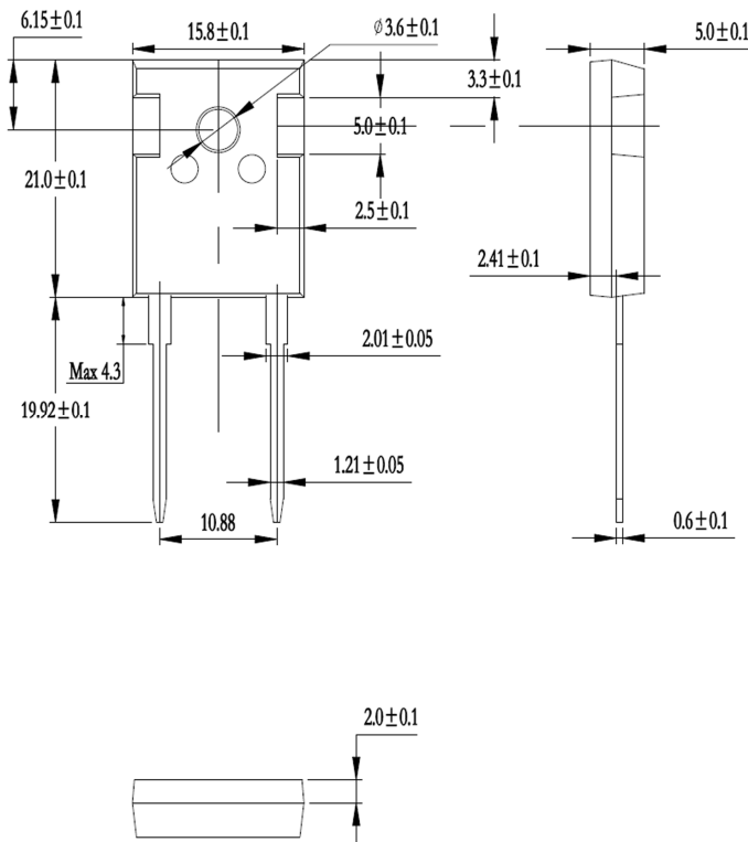
Dimensions in (mm) Figure 8. Package Outline
